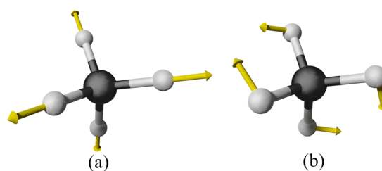
FIG. 5. (a) The symmetric stretch and (b) scissor vibrational modes of methane.
