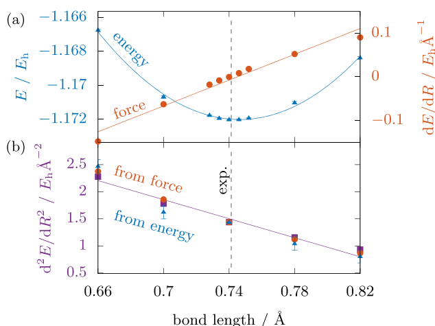
FIG. 2. (a) Energy, force, and (b) diagonal force constant against bond length, for the hydrogen molecule. For the energy and force plots, the parabolic and linear curves of the best fit for the visible data are overlaid. For the force constant plots, we show the diagonal force constant derived using the finite difference method from the energy curvature, the force gradient, and the direct analytical evaluation of the force constant. The line of the best fit for the visible MFC data is overlaid. The dashed line indicates the experimental equilibrium bond length. Error bars for all of the data are given—some error bars are smaller than the data points on the scale of the plot.
