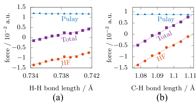
FIG. 1. Interatomic force estimates for the molecules (a) \text{H}_2 and (b) \text{CH}_4 . The red dots correspond to the Hellmann-Feynman (HF) force, the blue triangles correspond to the Pulay force, and the magenta squares correspond to the total force. Error bars for all of the data are given—some error bars are smaller than the data points on the scale of the plot.
