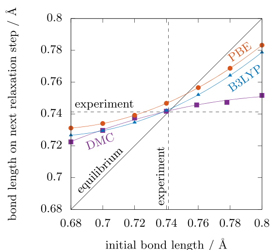
FIG. 3. Bond length on the next step of atomic relaxation as a function of initial bond length, for the hydrogen molecule. The unconstrained parabolas of the best fit, with respect to the visible DFT (PBE, B3LYP) and DMC data points, are overlaid. The dashed lines indicate the experimental equilibrium bond length, whereas the solid line indicates the equilibrium fixed points with respect to the plot. DMC error bars are smaller than the data points on the scale of the plot.
